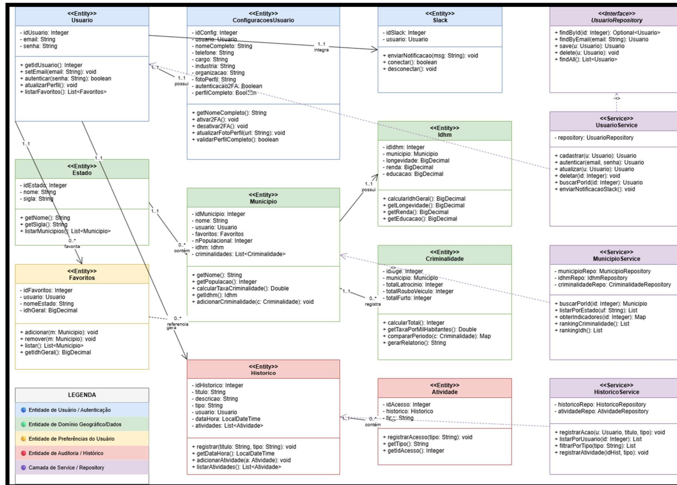
Figura 36 – Diagrama de classes da Safety Intelligence.
